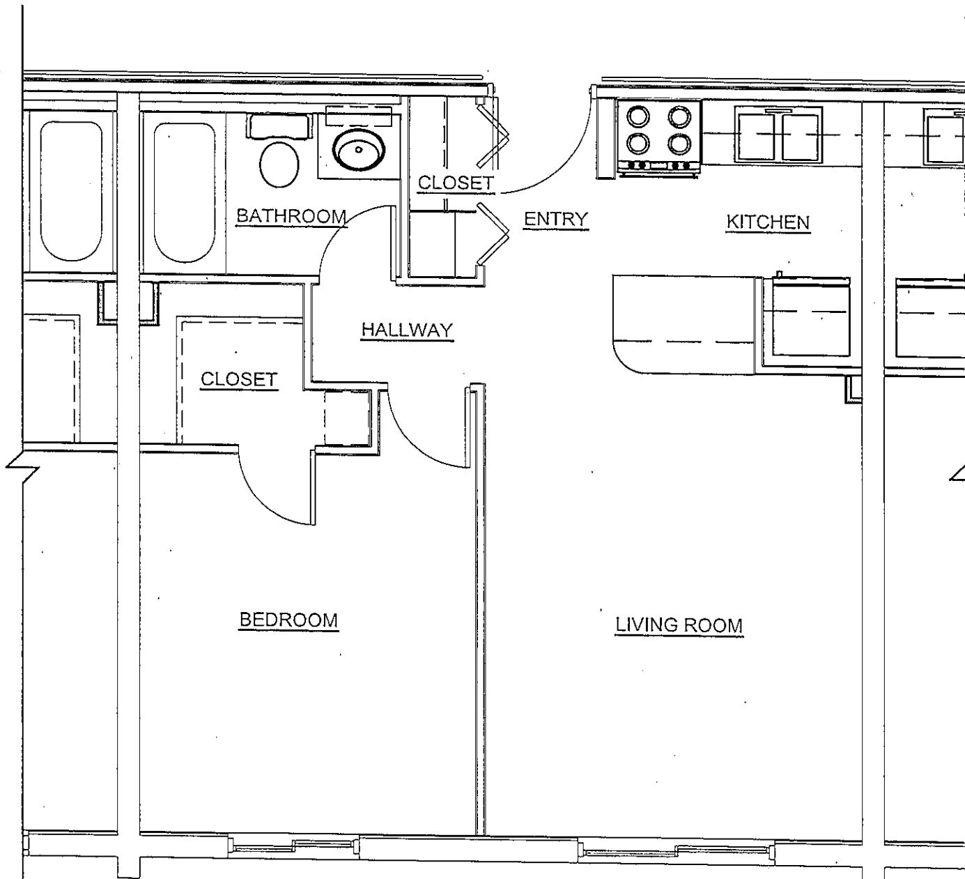
1 ONE BEDROOM UNIT SK-1 SCALE: 1/4" = 1'-0"
